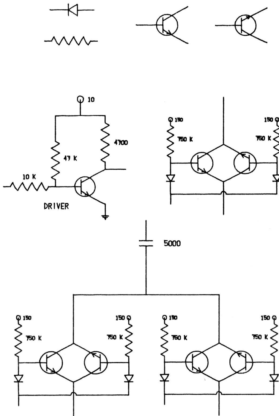
FIGURE 9.11. CIRCUIT DIAGRAMS
