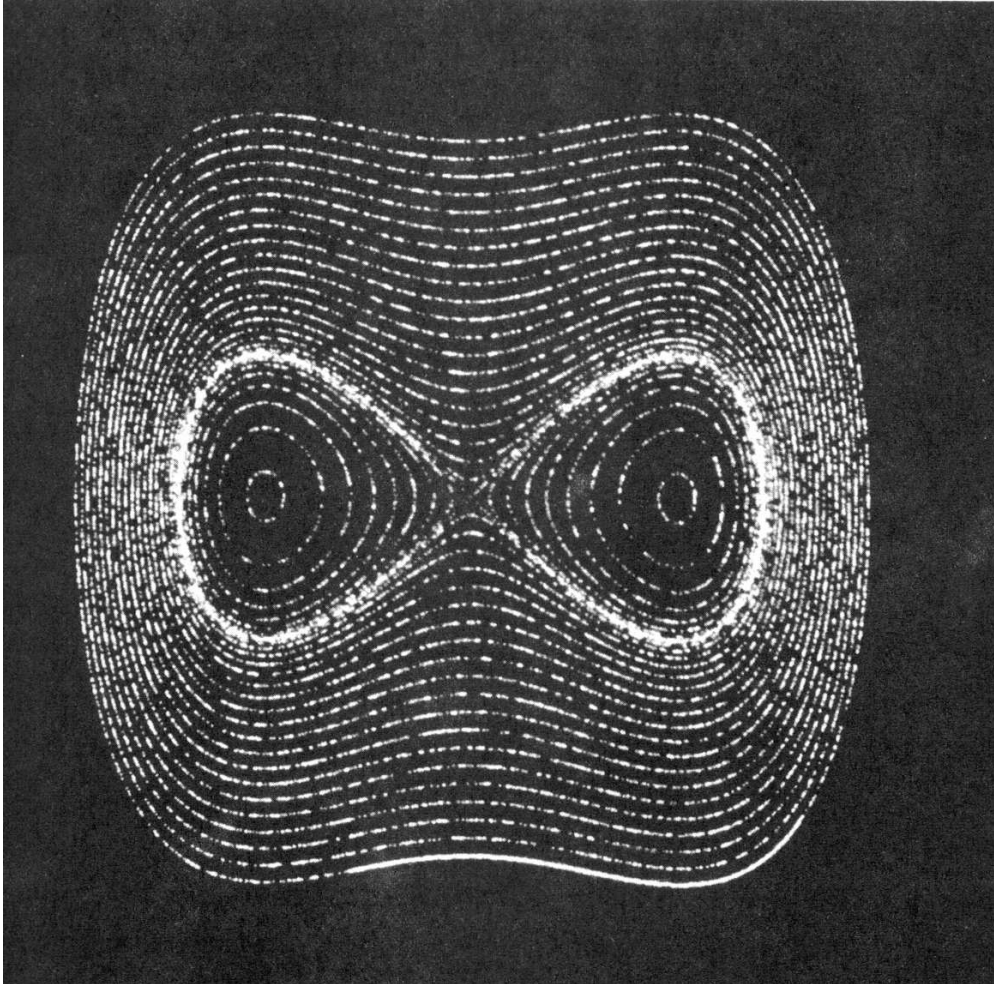
Figure 5.1: TWINKLING DISPLAY. Displaying the spots of a large display in random sequence makes the display appear to “twinkle.” This photograph was exposed only long enough to show about half of the spots of a twinkling display. It conveys the impression of a twinklings display as well as any still picture can.
