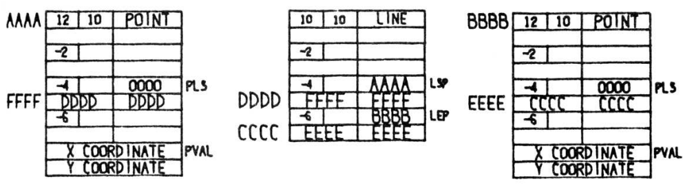
FIGURE 3.3. LINE SEGMENT AND END POINTS IN RING STRUCTURE NOTATION
