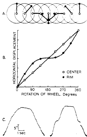
Fig. 3. A: Locus of points on the rim and hub of a wheel that rolls through one revolution. B: Horizontal displacement of points on the rim and hub of a wheel that rolls through 360^\circ . C: Typical horizontal eye movement records of a subject's attempts to track the centre of rotation through movement of wheel first to the left and then to the right. In the left trace two rim lights diametrically opposed were visible; in the right trace only one rim light was on. In both instances the lights traversed cycloidal paths (as depicted in the rim path in B), but when two cycloids 180^\circ out of phase were present, the subject perceived a rotating wheel and was able to track the imagined centre. With only one rim light on, no percept of a rolling wheel was formed and the subject resorted to tracking that single light through the cycloid path.
