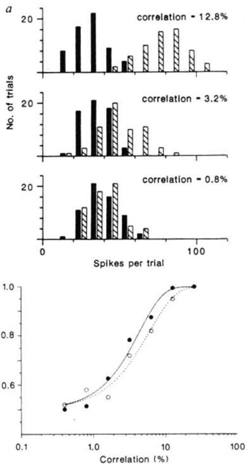
FIG. 1 Physiological and psychophysical data obtained simultaneously from a rhesus monkey. a The responses of a directionally selective MT neuron at three different motion correlations spanning physiological threshold. The hatched bars represent responses to motion in the neuron's preferred direction; the solid bars indicate responses to motion in the null direction (180° opposite to the preferred). Sixty trials were performed in each direction for each of the three correlation levels. Response distributions for a range of correlation levels were used to compute a 'neurometric' function that characterized the neuron's sensitivity to the motion signal and could be compared with the psychometric function computed from the monkey's behavioural responses. b Comparison of simultaneously recorded psychometric and neurometric functions. Psychophysical performance of the monkey, ○; performance of the neuron, ●. Psychophysical performance at each correlation is given by the proportion of trials on which the monkey correctly identified the direction of motion. Neuronal performance is calculated from distributions of responses like those in Fig. 1 a using a signal-detection method described in the text. The physiological and psychophysical data form similar curves, but the data for the neuron lie to the left of the data for the monkey, meaning that the neuron was somewhat more sensitive than the monkey. We fit the data with smooth functions of the form introduced to psychophysics by Quick 12 . Threshold, defined as the correlation for which the direction of motion was identified correctly on 82% of the trials, was 6.1% for the monkey and 4.4% for the neuron.
