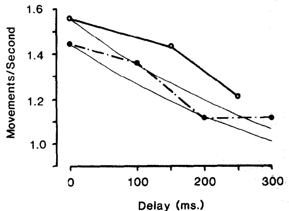
Fig. 6. Examples of fall in monkey's average rate of positional corrections when tracking a pseudo-random waveform with visual feedback delays (dark lines); predicted rates of movements are given by the light lines.
