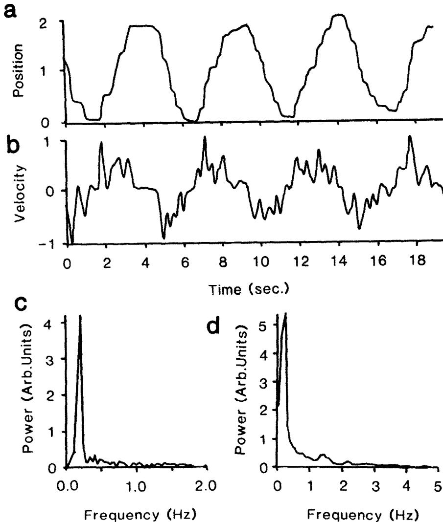
Fig. 1. Response of a monkey tracking a 0.2 Hz sinusoidal target (not shown). Step-and-hold movements can be seen in the position record (a), and appear as discrete peaks in the velocity record (b). c: 1024 point FFT power spectrum of Fig. 1a. The large peak is at the target frequency, little power is associated with the step-and-hold movements. d: an average autoregressive spectrum calculated by averaging twenty 256 point spectra triggered off the target signal; note the peaks at 1.5 and 2.2 Hz.
