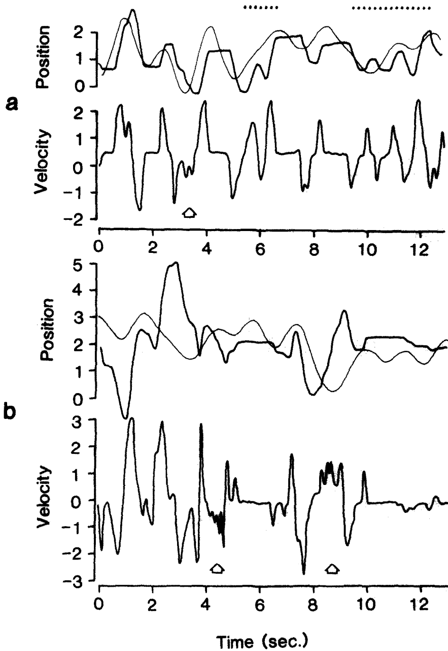
Fig. 8. Human responses (heavy lines) when tracking with long visual feedback delays. a: Brief "hunting" (dotted periods) about the target waveform (light line); delay 200 ms. b: Brief periods of high frequency corrections (arrows); delay 300 ms.
