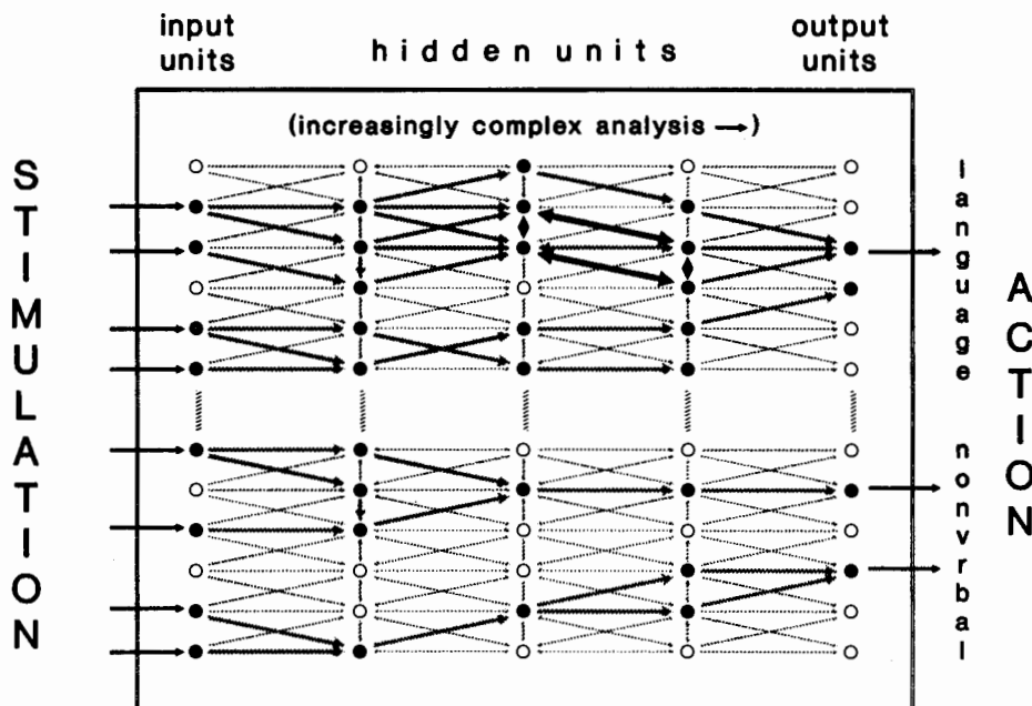
Figure 2 Representation of Conscious and Unconscious Cognition in the Format of Neural Network (Connectionist, or Parallel Distributed Processing) Models
