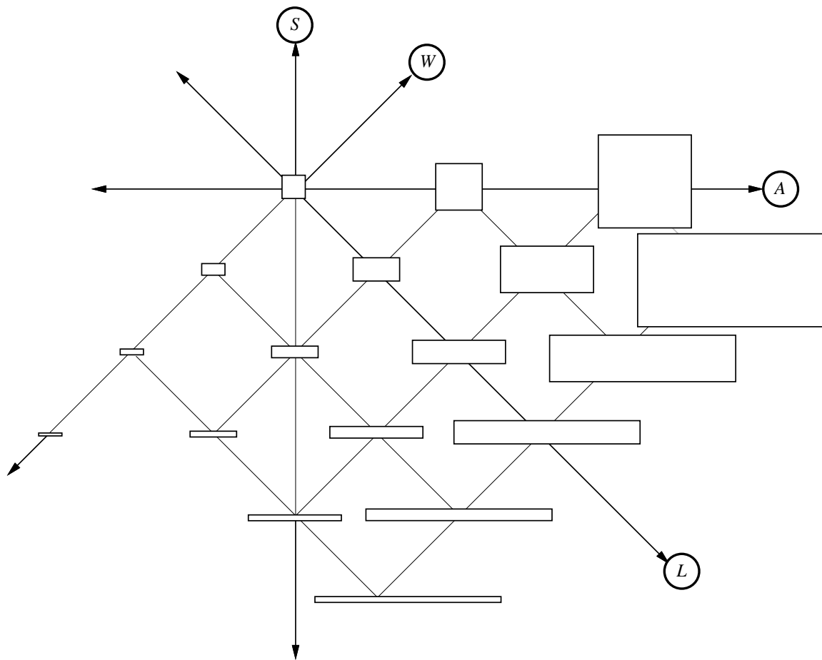
Figure 3: Rectangle space, showing how the \langle L, W \rangle coordinate systems is 45^\circ rotation of the \langle A, S \rangle system. As A increases (“east”), area increases while shape remains constant; as S increases (north), the rectangle becomes more square, while the area remains constant; as W increases (north-east), the shorter dimension grows; while as L increases (south-east) the longer dimension grows. The rectangles shown are the ones used in the experiments.
