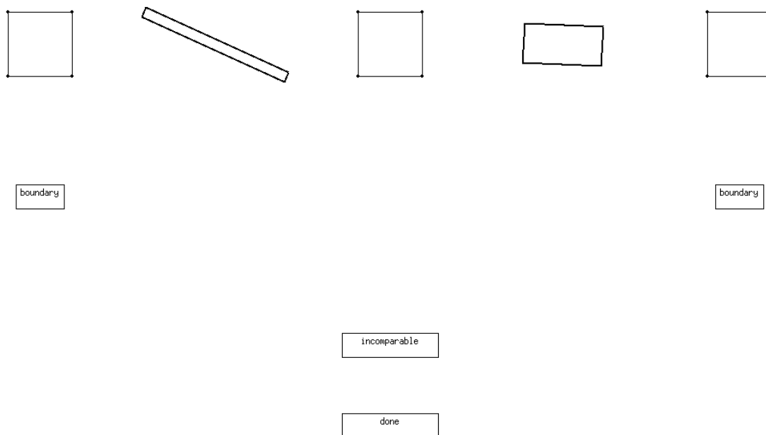
Figure 2: A typical trial screen, containing the two fixed rectangles R_1 and R_2 , and three squares that subjects could manipulate with the mouse to construct the left extrapolant x , the interpolant y and the right extrapolant z .
