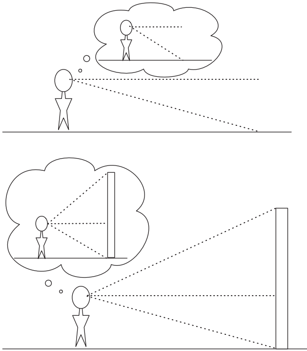
Figure II.16-4. (a) Independent of the presence of a ground surface, perceived gaze declination (within 45^\circ of horizontal) is exaggerated by a gain of 1.5 (Durgin & Li, 2011a; Li & Durgin, 2009). (b) Asked to set themselves the same distance from a pole as the pole is high, participants set themselves much too far away (Higashiyama & Ueyama, 1988). The mismatch between their perceptual experience and the physical situation can be predicted by the scaling of the perceived angular declination of gaze (Li et al., 2011).
