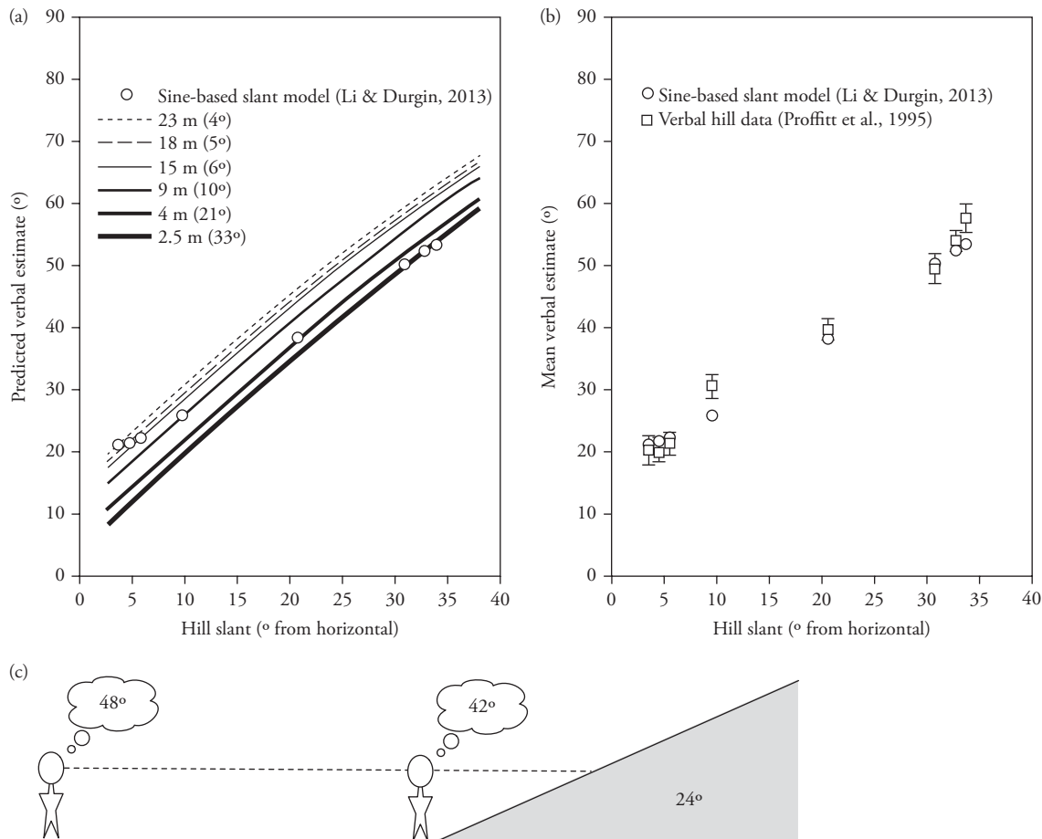
Figure II.16-2. For a farther observer, a hill will appear steeper. (a) An illustration of the empirically derived model of the effects of viewing distance on perceived slant (Li & Durgin, 2010, 2013). At each distance, slant judgments have a gain of about 1.5 (the function is primarily sinusoidal). (b) This one-parameter model fares well at predicting the hill estimation data of Proffitt et al. (1995): each white circle (in both graphs) represents the model prediction for a specific hill slant taking into account both its slant and the optical distance to hill for an observer at the base of the hill, viewing it with gaze forward. (c) The effect of distance generalizes to farther or nearer viewing: a hill of about 24^{\circ} will be estimated as 42^{\circ} when standing at the base (with gaze forward, the optical distance to the hill would be about 3.6 m) but as 48^{\circ} when standing 10 m back from the base (i.e., 13.6 m from the hill surface at eye level).
