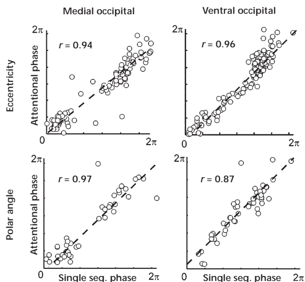
Fig. 2. Comparison of visual field topography (coded by temporal phase of fMRI response) for attentional foci ( y -axis) versus single segments ( x -axis). Each circle represents a single responsive voxel. Data are pooled across subjects. Left column, medial occipital cortex consisting primarily of V1 and V2. Right column, ventral occipitotemporal cortex within and surrounding the collateral sulcus. Top row, shifts in eccentricity. Bottom row, shifts in polar angle.
